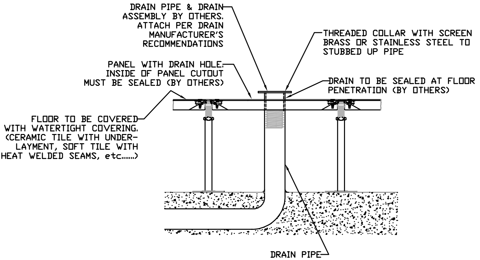
ELEVATION VIEW
